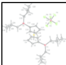
Fig. 1. The molecular structure of (I), showing ellipsoids at 30% probability level.
